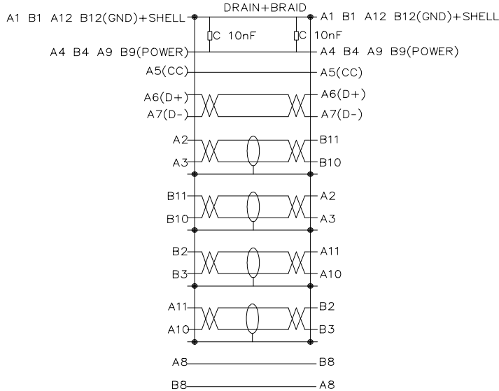
P1 Pin Assignment P2
